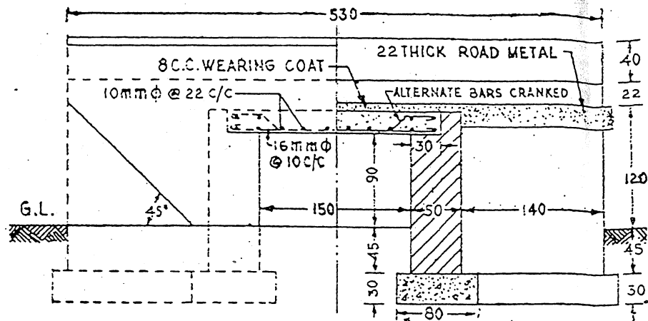
HALF SEC. ELEVATION ON ABCD
