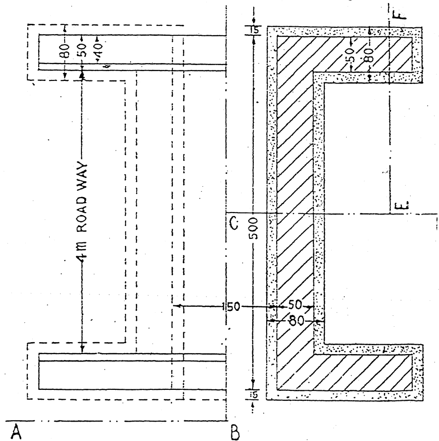
HALF SECTIONAL PLAN
