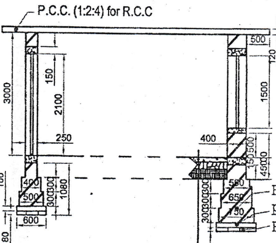
SECTION OF 0.25m, WALL
