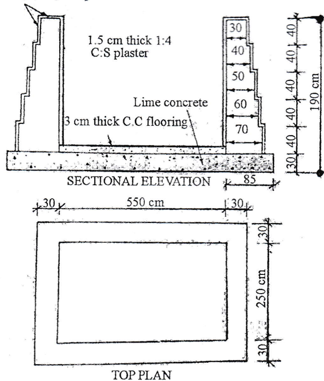
Fig: Underground Water tank
